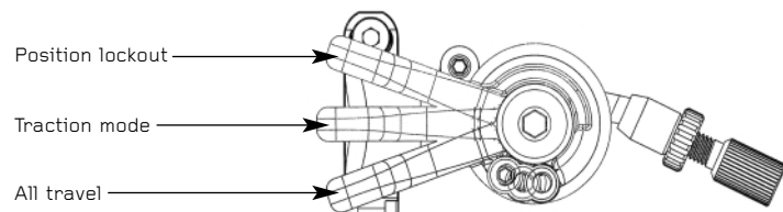
Traction Control-Functions
